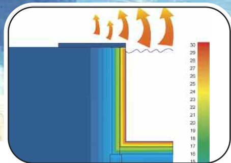
Thermapool™ saves 86% of heat loss
